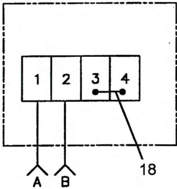
WIRING DETAIL
